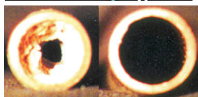
ScaleBlaster Model SB-75 (top) Scale in water pipe before (left) and after ScaleBlaster use
